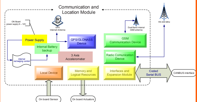
General diagram and functional architecture:
